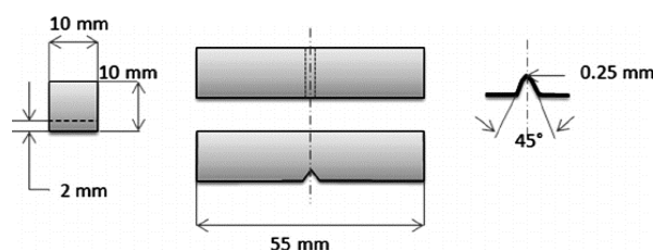
Fig. 1 Impact Specimen
