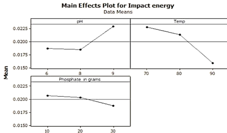
Fig. 4.5 Main Effects Plot for Impact Energy
