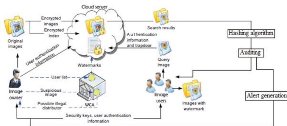
Fig. 1. Framework of the content-based image retrieval using watermark based protocol
