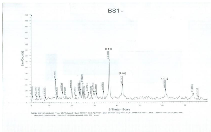
Fig: XRD of Copper nanopowder
