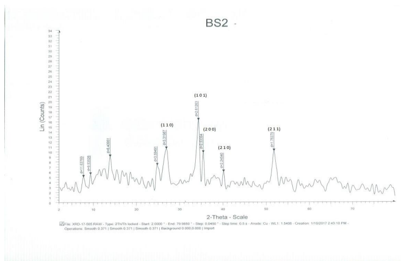
Fig: XRD of Cu doped SnO 2
