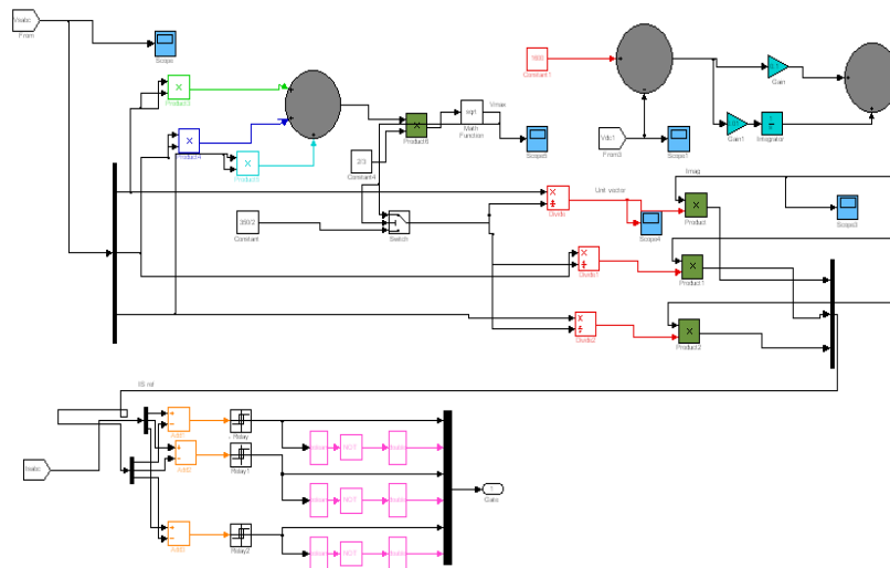
Fig. 8. Control Circuit
