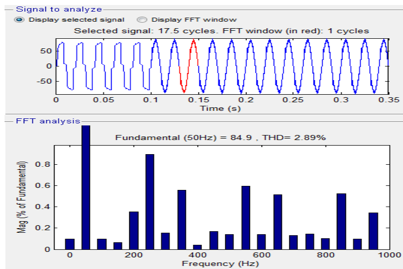
Fig.11 FFT Analysis of Phase A Source Current
