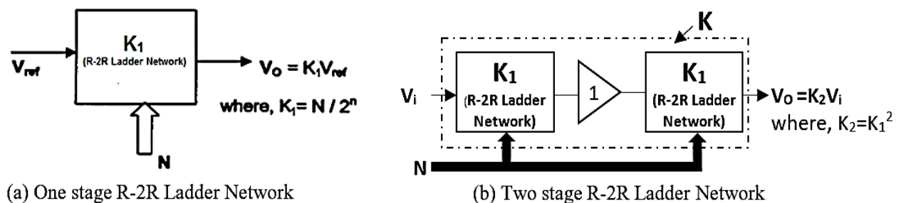
Fig. (4) Block Diagrams of R-2R Ladder Networks
