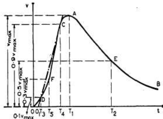
Fig 1. General impulse waveform
