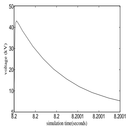
Figure 6. Multistage impulse waveform, 45KV, 1.2/50 \mu sec.
