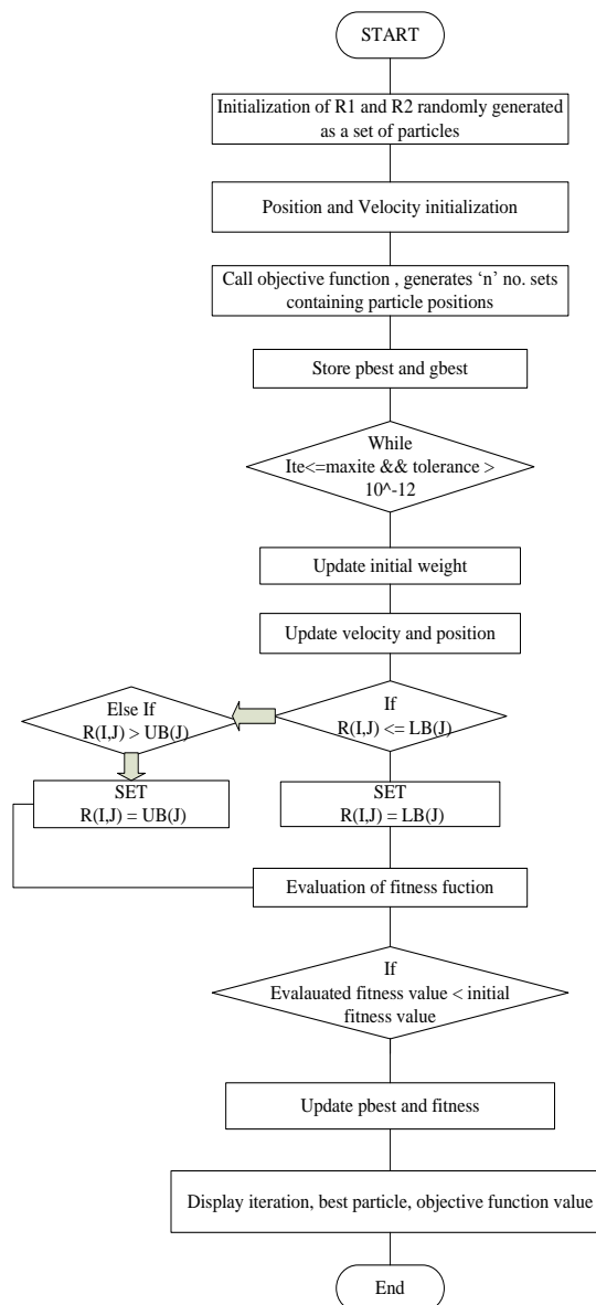
Fig 4. Flowchart for particle swarm optimization
