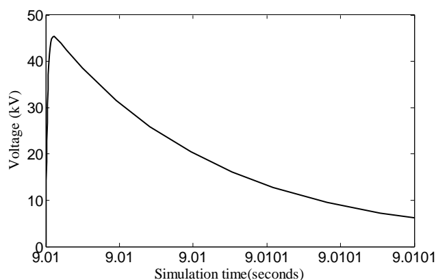
Figure 5. Single stage impulse waveform, 45KV, 1.2/50 \mu sec.
