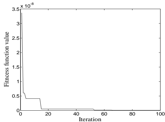
Figure 3. PSO convergence characteristics for the best run
