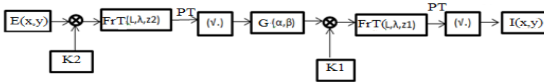
Fig. 1(b) Decoding scheme
