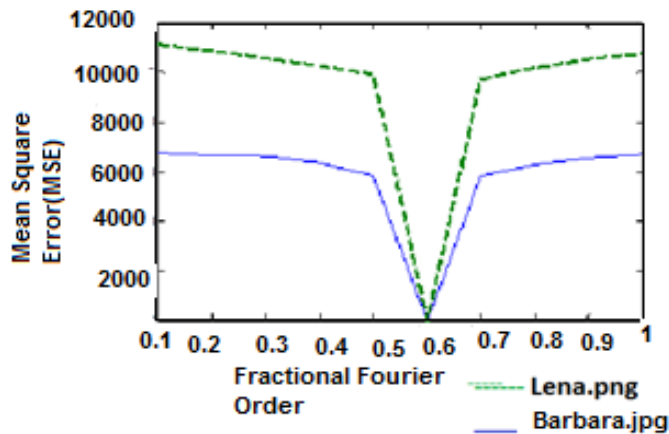
Fig. 3 Plot of MSE against Fractional order
