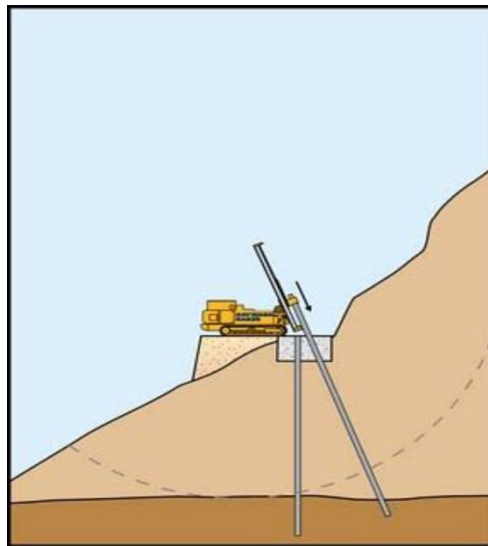
Figure 2. In-Situ Reinforcement
