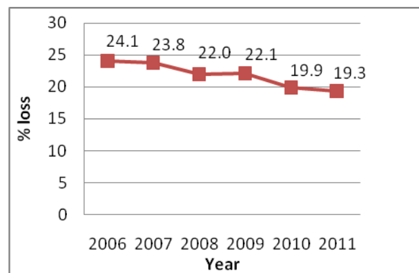
Fig 1. Variation of Losses in Distribution System in Yangon
